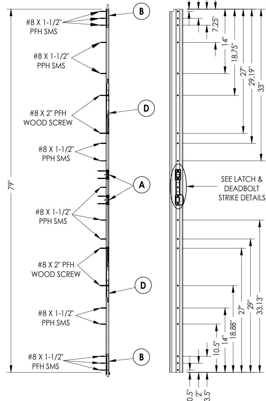
HURRICANE ASTRAGAL ASSEMBLY
