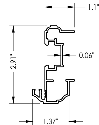
35 ALUMINUM ASTRAGAL
