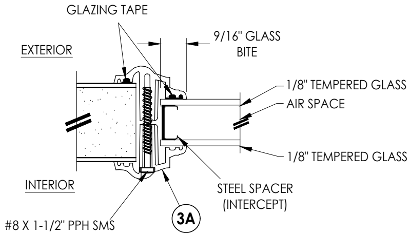
G1 GLAZING DETAIL ODL LITE FRAME
