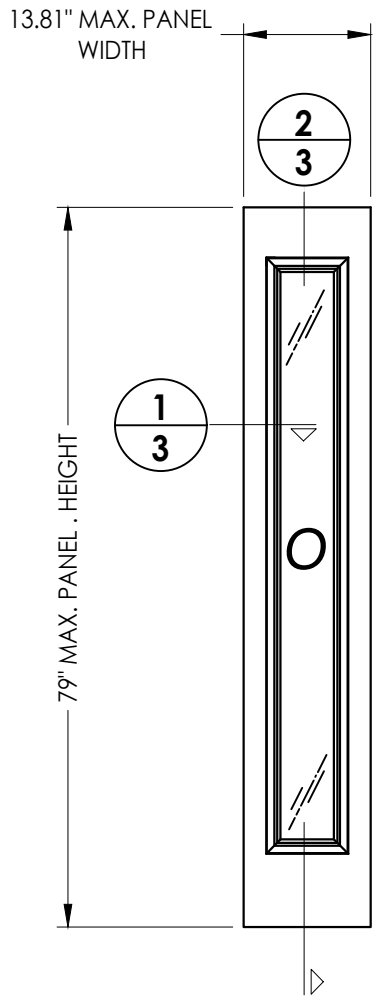
50 STEEL SIDELITE PANEL ODL, INC.
