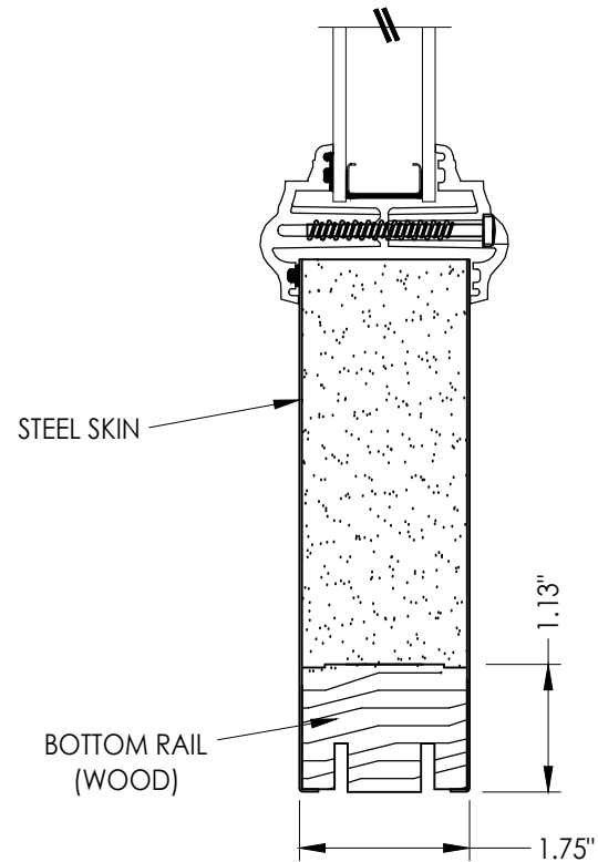
2 2 VERTICAL CROSS SECTION
