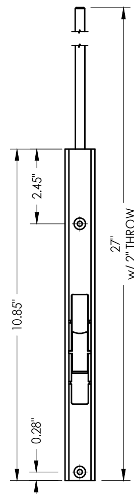
D SLIDE LOCK FLUSHBOLT ASSEMBLY HURRICANE ASTRAGAL
