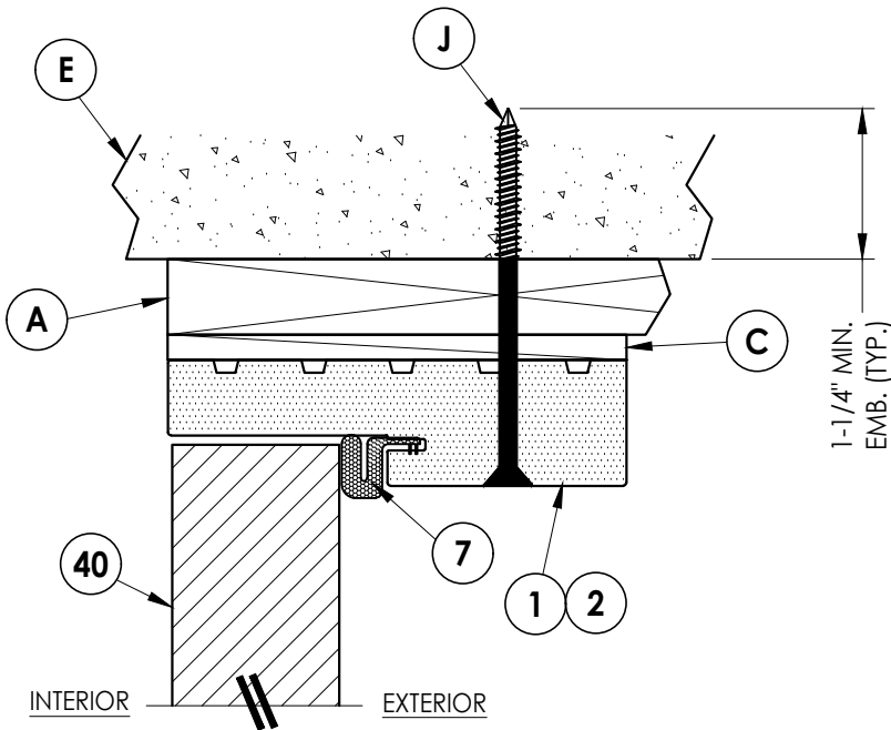
3 VERTICAL CROSS SECTION 6 Inswing Shown (Outswing Similar) 1X Buck Construction
