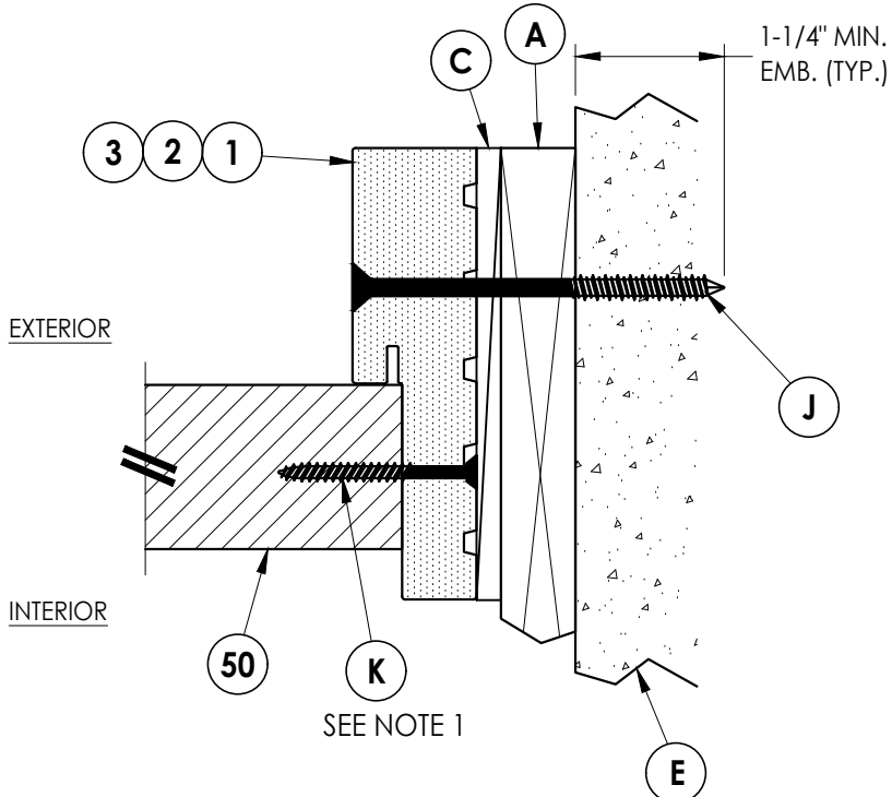
2 HORIZONTAL CROSS SECTION 6 Inswing Shown (Outswing Similar) 1X Buck Construction
