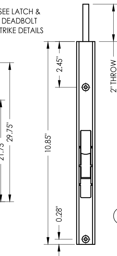
SLIDE LOCK FLUSHBOLT ASSEMBLY STANDARD ASTRAGAL
