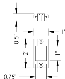
A STOP BRACKET
