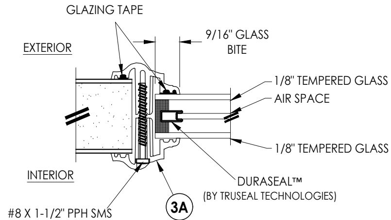
G2 GLAZING DETAIL ODL LITE FRAME
