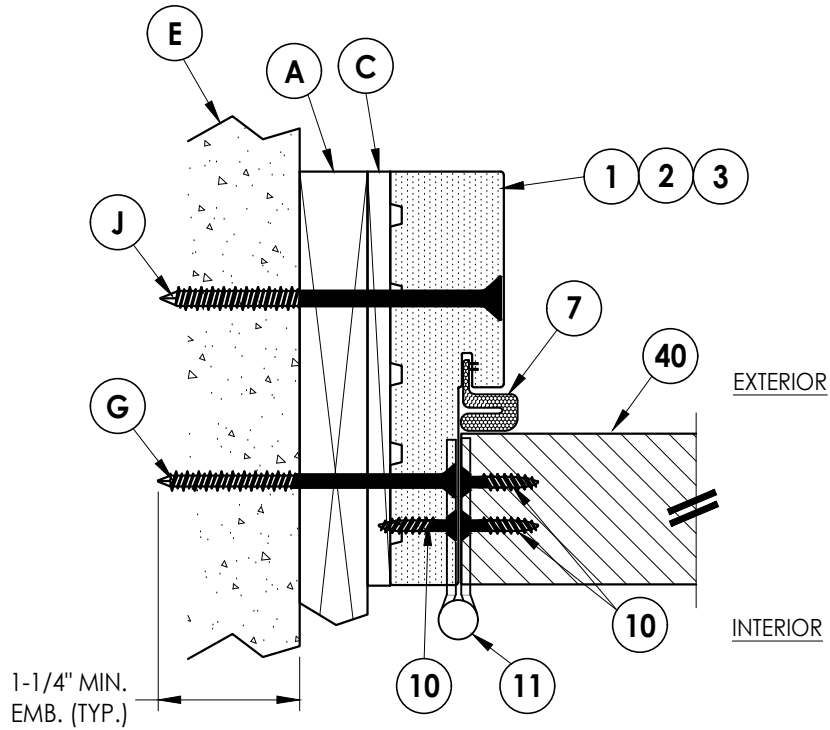
1 HORIZONTAL CROSS SECTION 6 Inswing Shown (Outswing Similar) 1X Buck Construction
