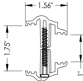
3A ODL LITE FRAME EVOLVE FRAME HP POLYPROPYLENE
