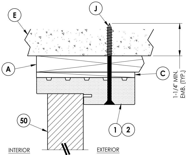
4 VERTICAL CROSS SECTION 6 Inswing Shown (Outswing Similar) 1X Buck Construction
